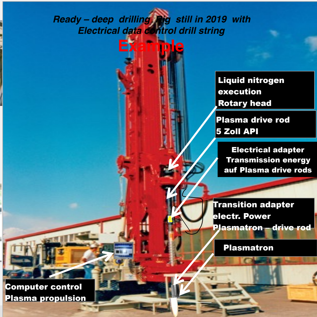
Electrical superconductors Plasma drive rod 5" API
