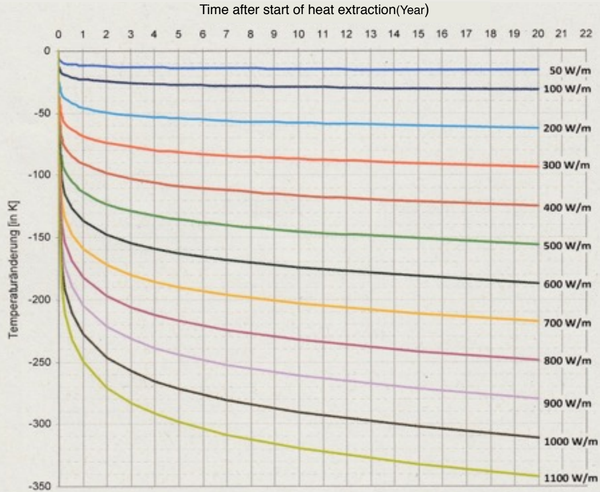
Illustration: Temperature drop at the borehole wall at different power densities
